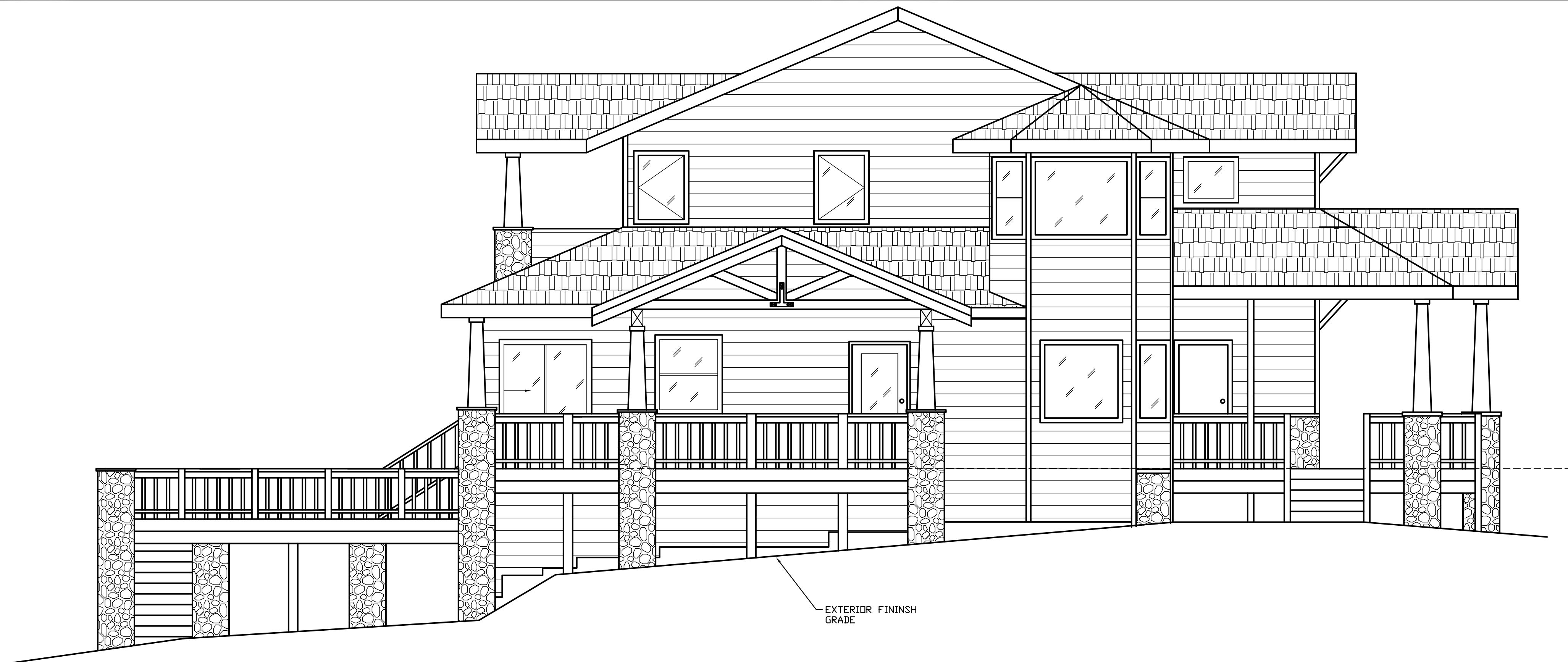
LEFT ELEVATION
