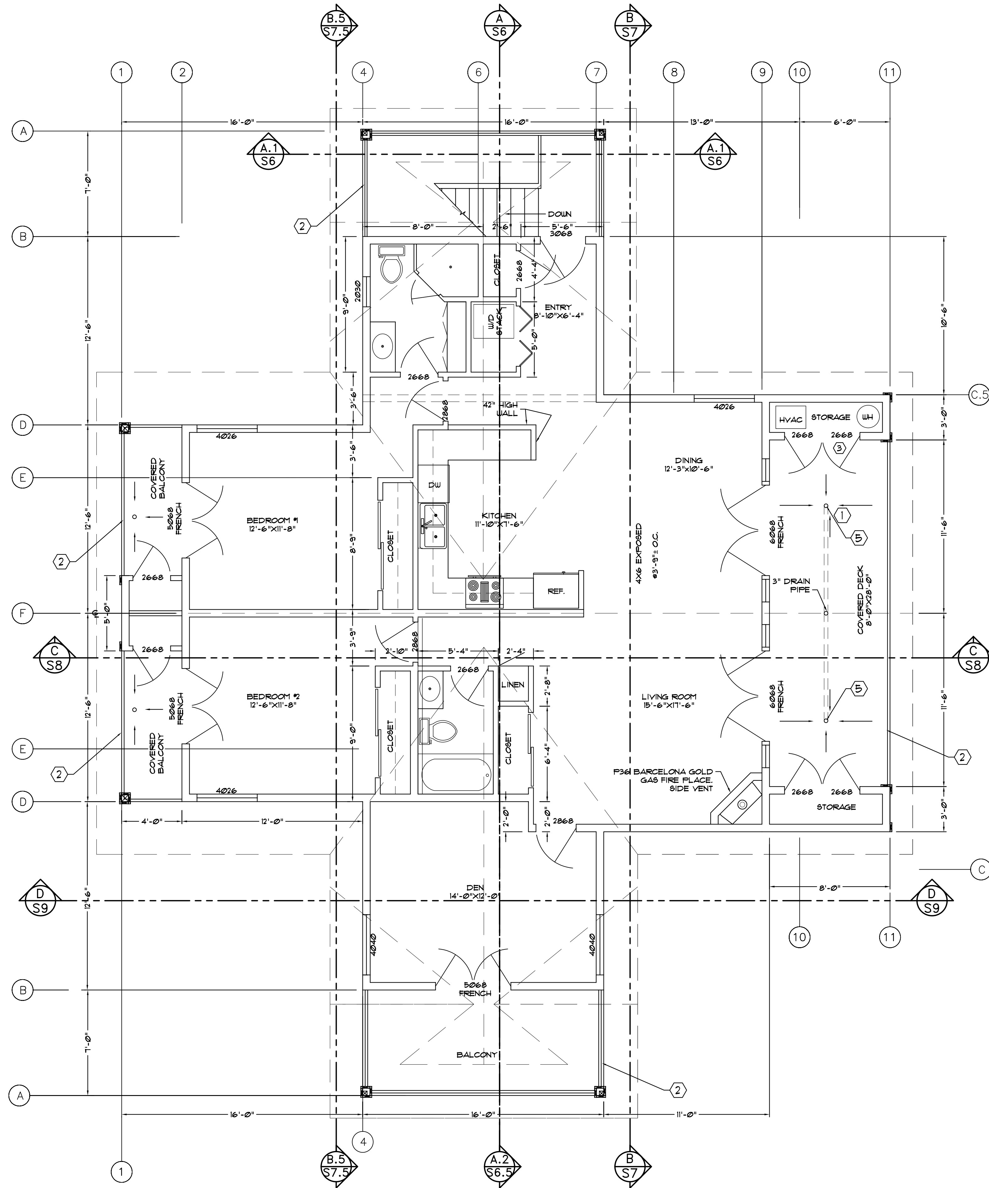
PENTHOUSE FLOOR PLAN SCALE: 1/4" = 1'-0" 1394 SF.
